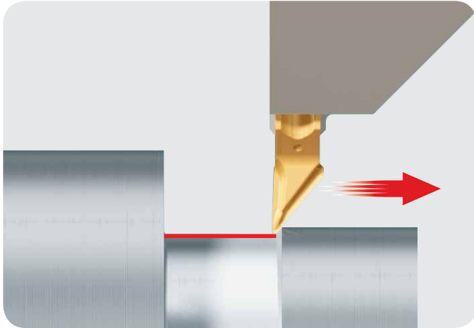
Backward turning
